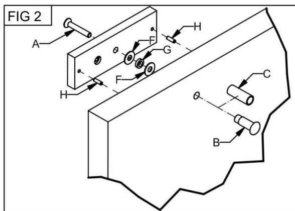
ASSEMBLED ELECTRO MAGNET
