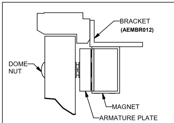
ASSEMBLED ELECTRO MAGNET
